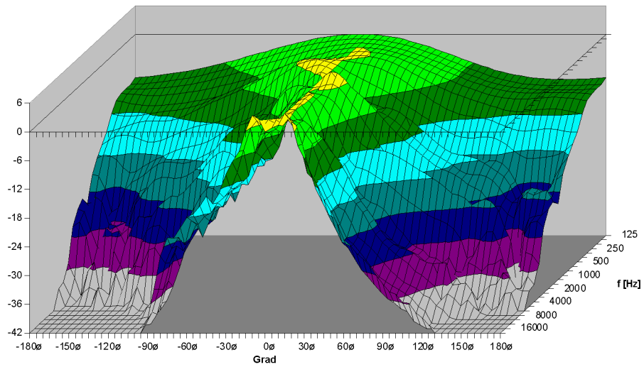
TSM 15 Vertikal - 3D Directivity Plot
