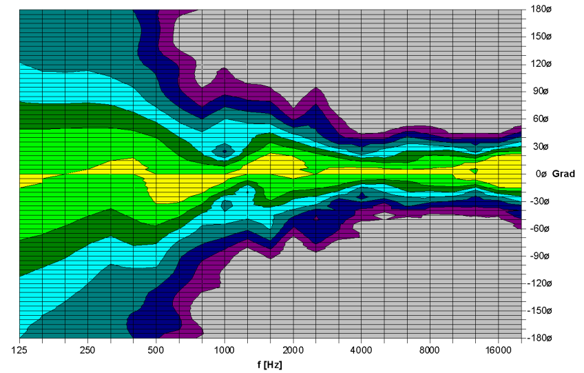
TSM 15 Vertikal - 2D Directivity Plot
