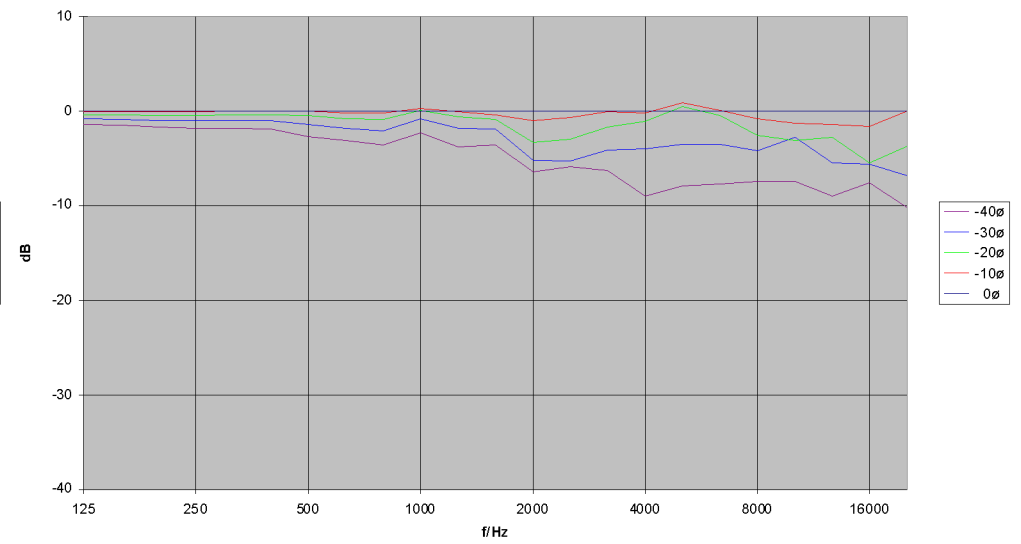
TSM 15 Horizontal - Frequenzgang Off Axis (-)
