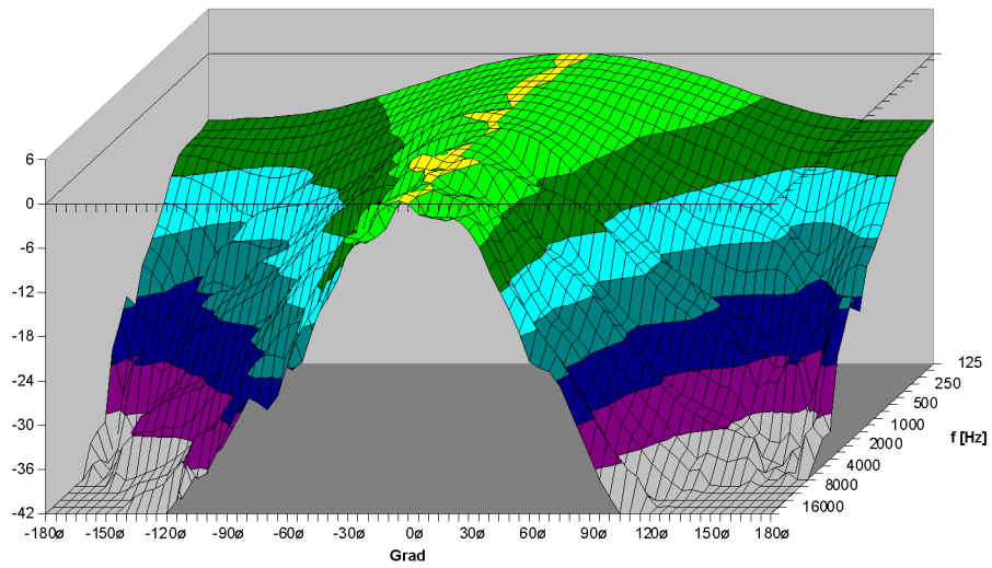
TSM 15 Horizontal - 3D Directivity Plot
