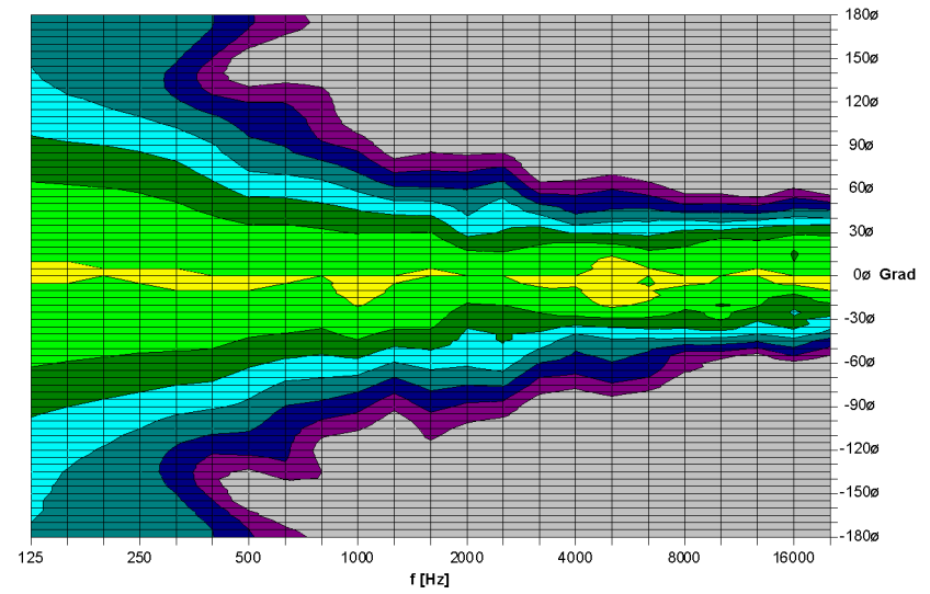
TSM 15 Horizontal - 2D Directivity Plot
