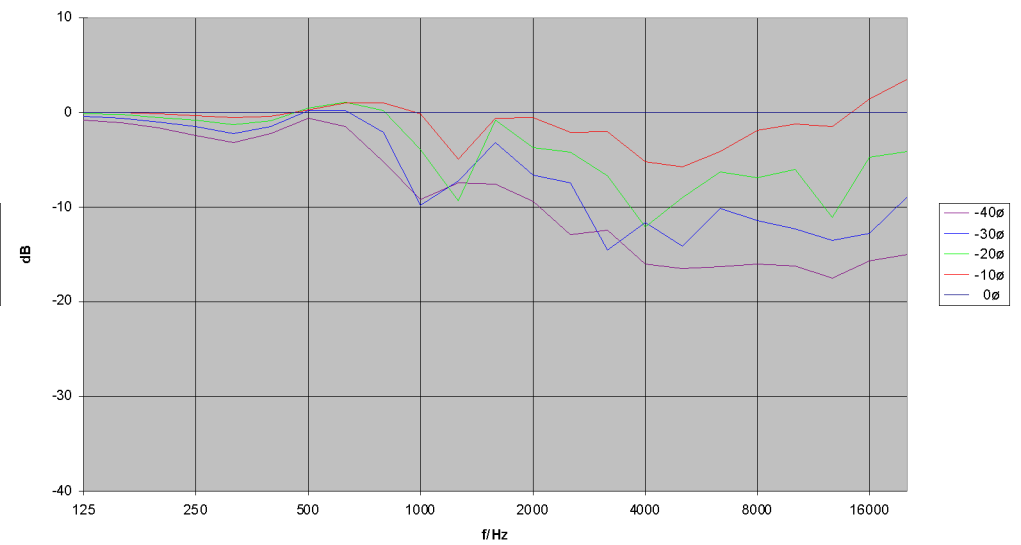
TSM 15 Vertikal - Frequenzgang Off Axis (-)
