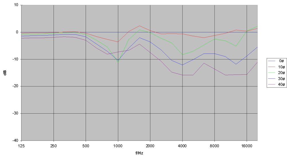
TSM 15 Vertikal - Frequenzgang Off Axis (+)
