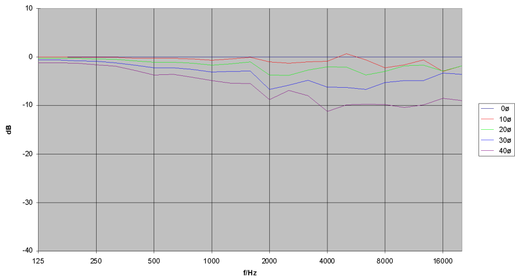
TSM 15 Horizontal - Frequenzgang Off Axis (+)
