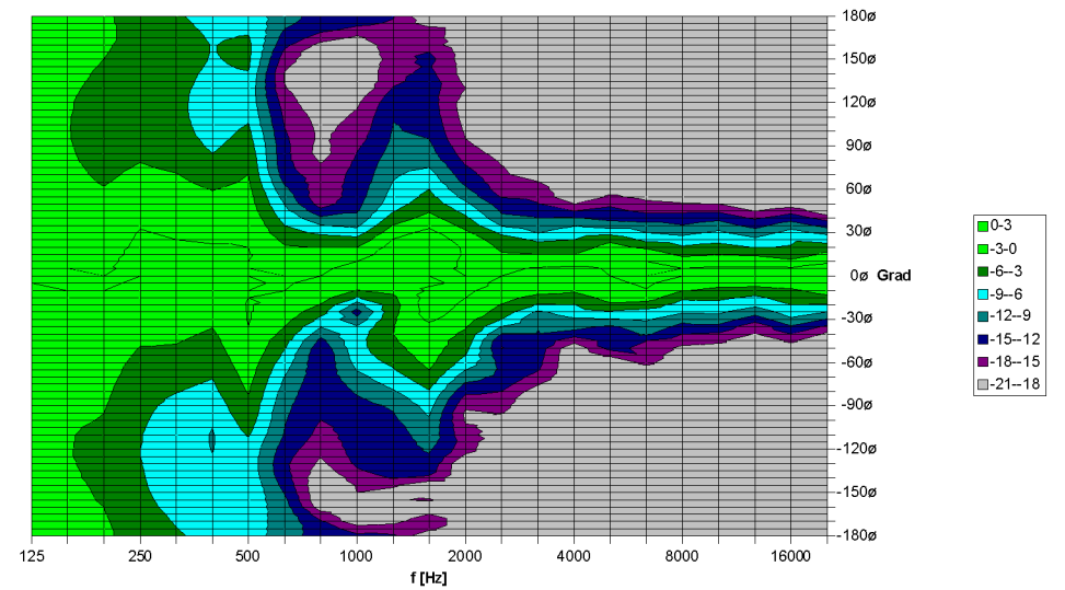
TSM12 90° x 60° Vertikal - Directivity Plot
