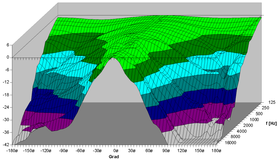
TSM12 90° x 60° Horizontal - 3D Directivity Plot
