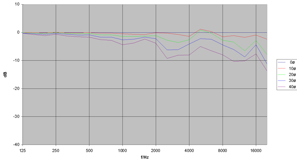
TSM12 90° x 60° Horizontal - Frequenzgang Off Axis
