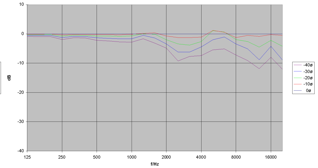
TSM12 90° x 60° Horizontal - Frequenzgang Off Axis
