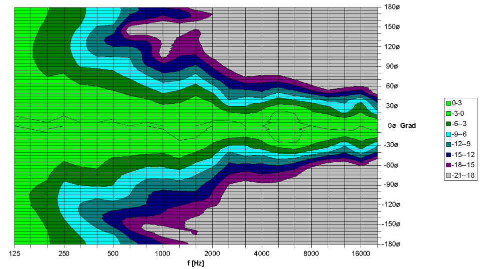
TSM12 90° x 60° Horizontal - Directivity Plot
