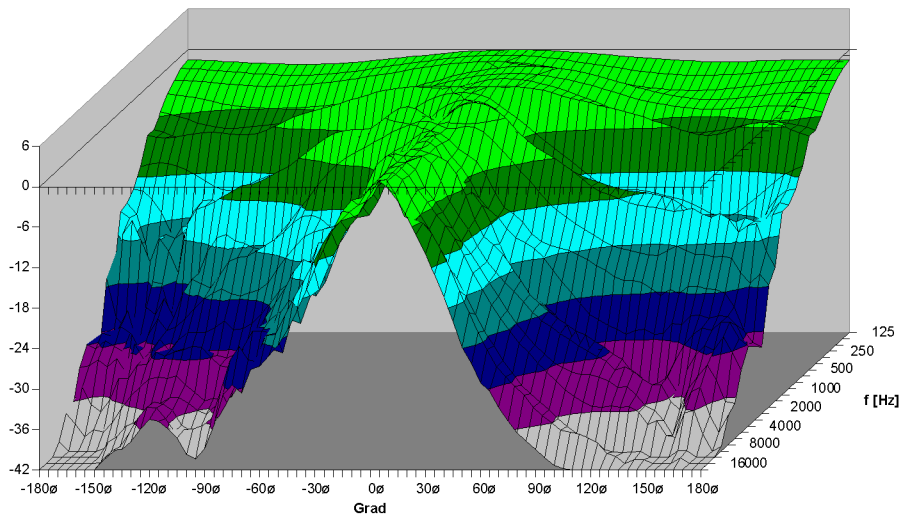
TSM12 90° x 60° Vertikal - 3D Directivity Plot
