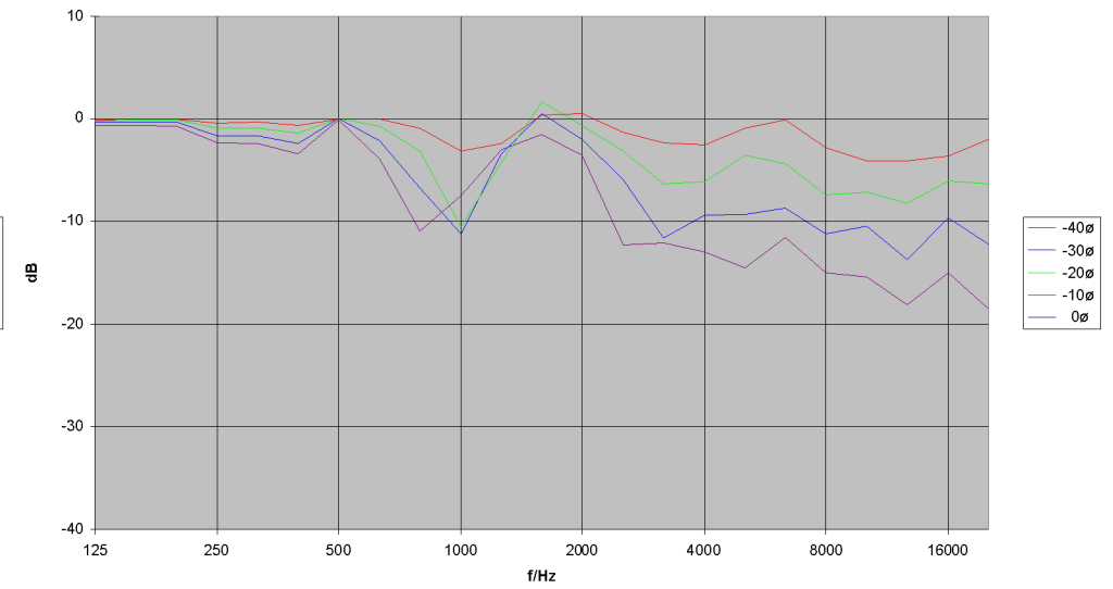
TSM12 90° x 60° Vertikal - Frequenzgang Off Axis
