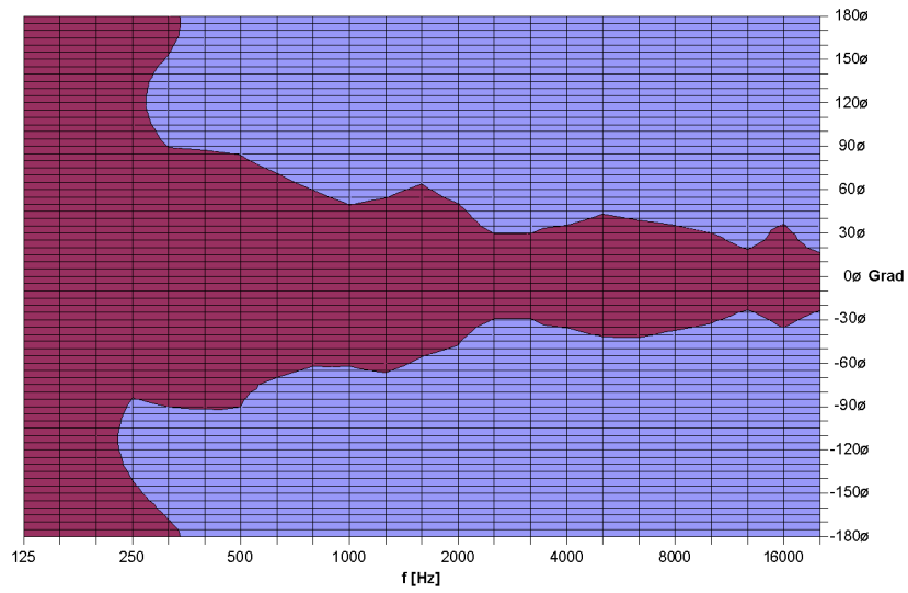
TSM12 90° x 60° Horizontal - -6 dB Isobaren
