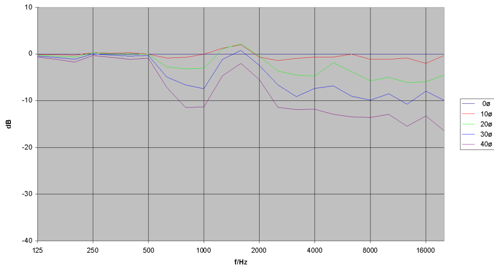
TSM12 90° x 60° Vertikal - Frequenzgang Off Axis
