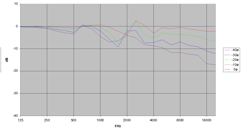
TSM 10 Vertikal - Frequenzgang Off Axis (-)
