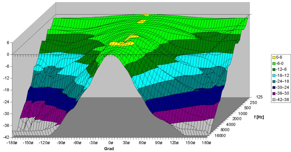
TSM 10 Horizontal - 3D Directivity Plot
