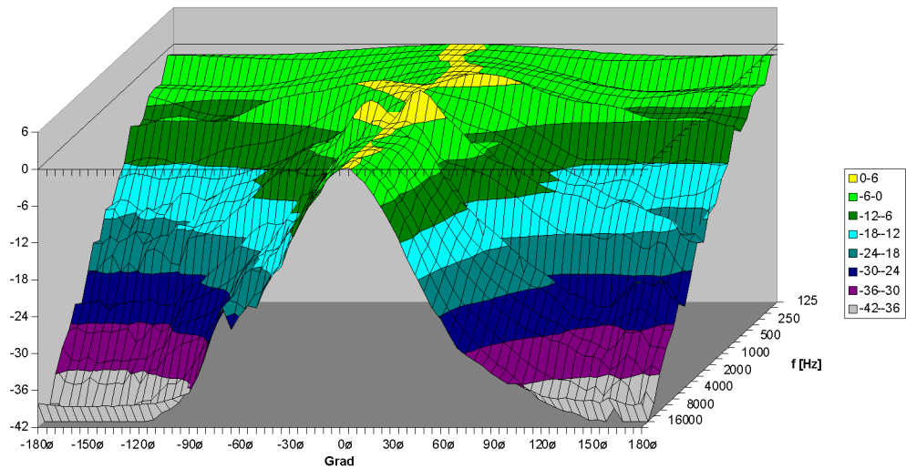
TSM 10 Vertikal - 3D Directivity Plot
