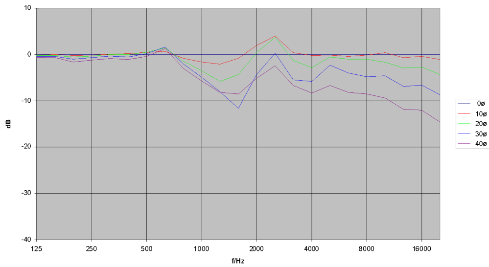
TSM 10 Vertikal - Frequenzgang Off Axis (+)
