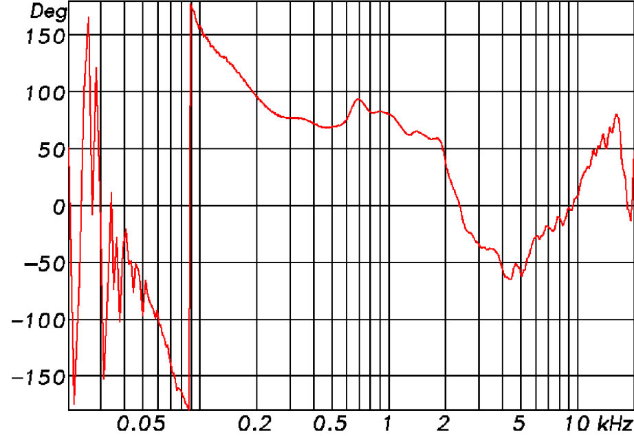
Phase Resp. TSM10
