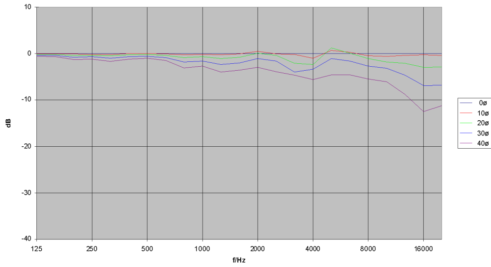
TSM 10 Horizontal - Frequenzgang Off Axis (+)
