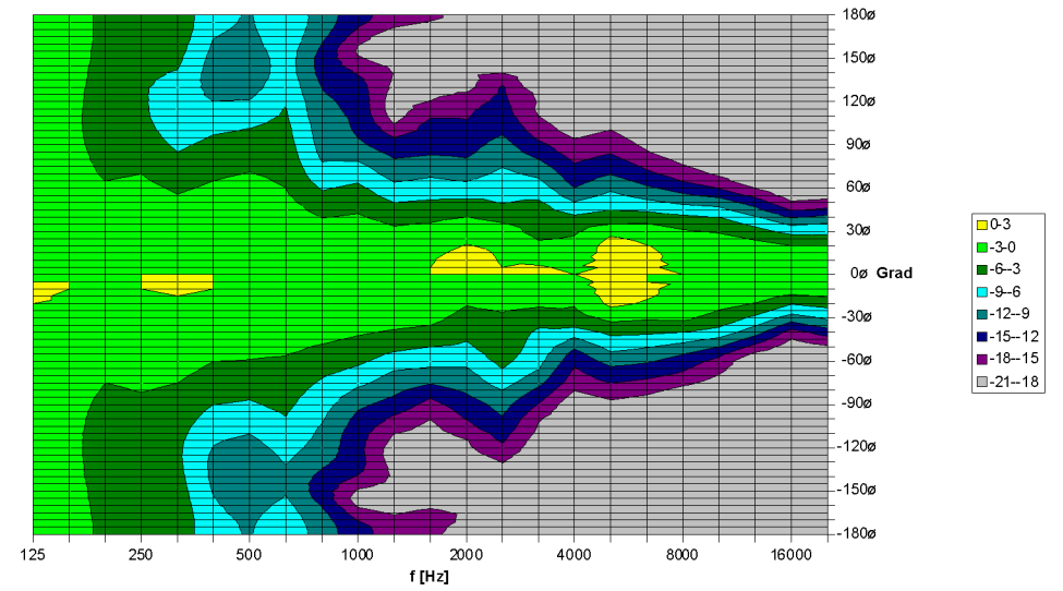
TSM 10 Horizontal - 2D Directivity Plot
