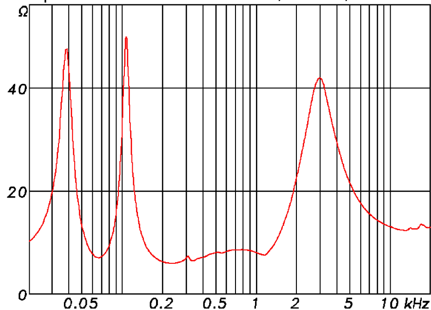
Impedance TSM10 Norm.= 8 Ohm ; Min.= 6, 0 Ohm
