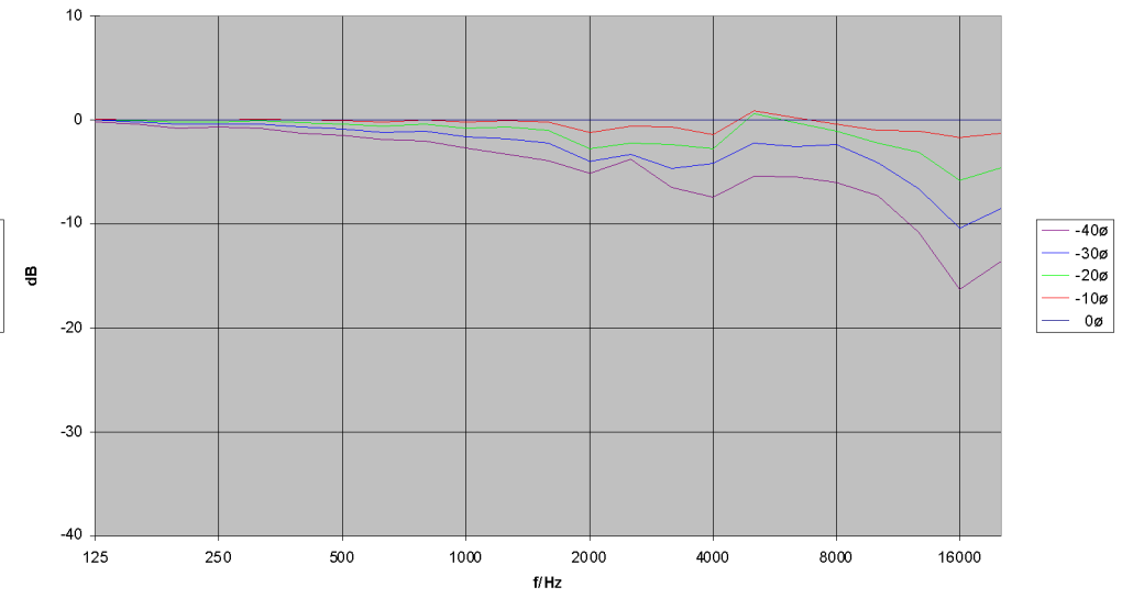
TSM 10 Horizontal - Frequenzgang Off Axis (-)
