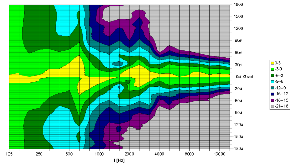
TSM 10 Vertikal - 2D Directivity Plot
