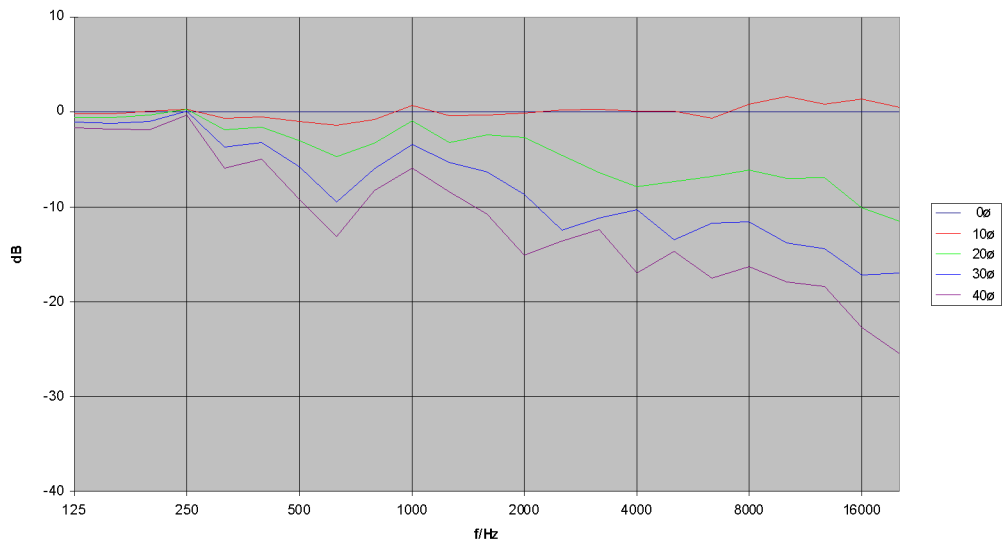
TSE 4030 Vertikal - Frequenzgang Off Axis (+)
