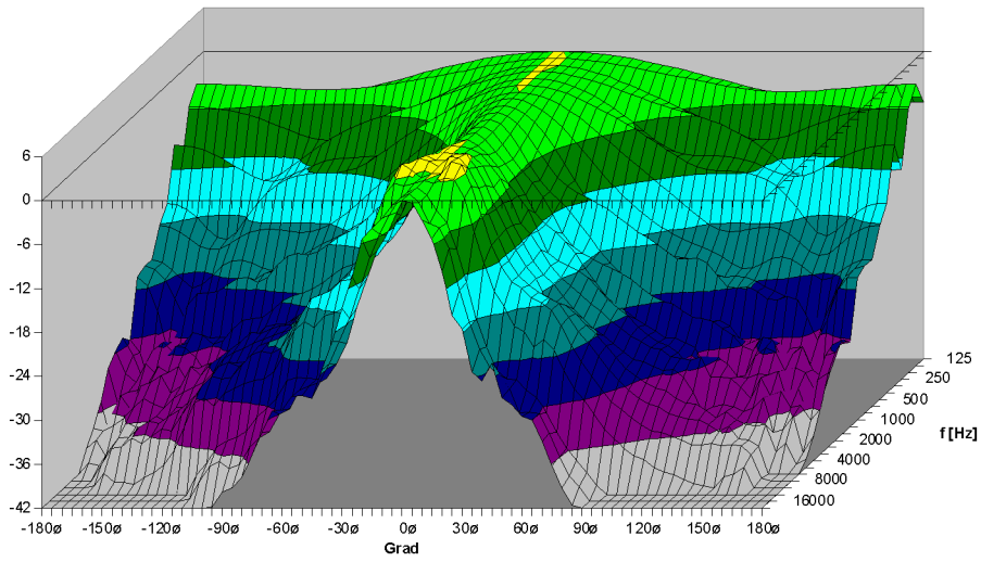
TSE 4030 Horizontal - 3D Directivity Plot
