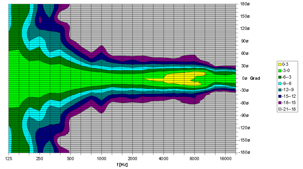
TSE 4030 Horizontal - 2D Directivity Plot
