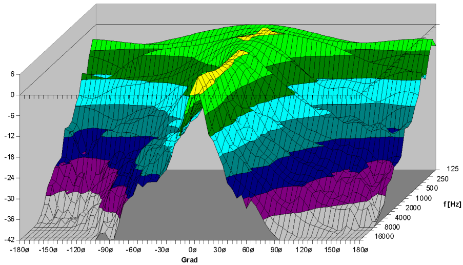
TSE 4030 Vertikal - 3D Directivity Plot
