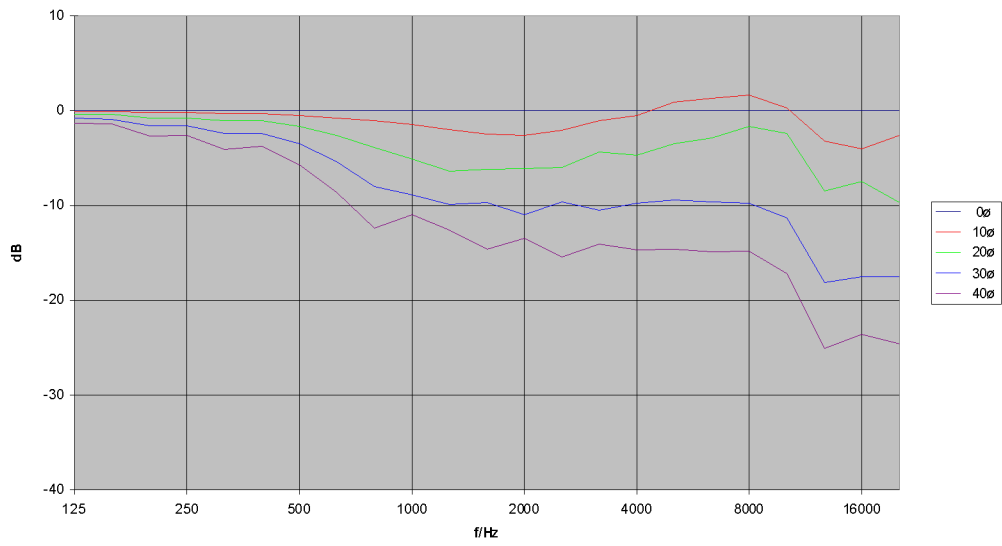
TSE 4030 Horizontal - Frequenzgang Off Axis(+)
