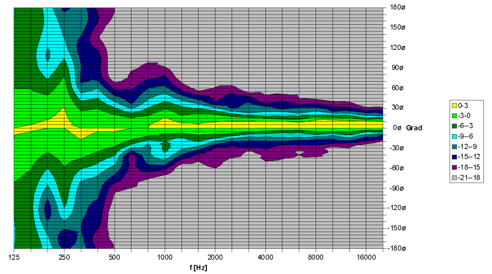
TSE 4030 Vertikal - 2D Directivity Plot
