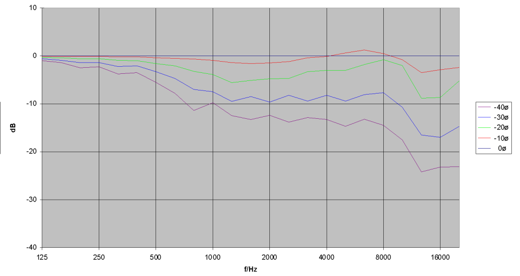
TSE 4030 Horizontal - Frequenzgang Off Axis(-)
