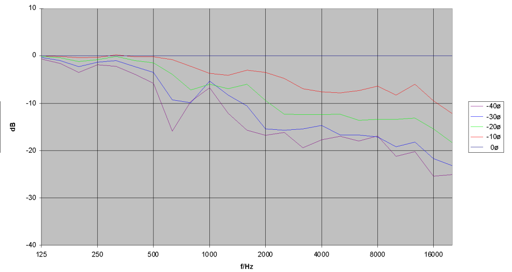
TSE 4030 Vertikal - Frequenzgang Off Axis (-)
