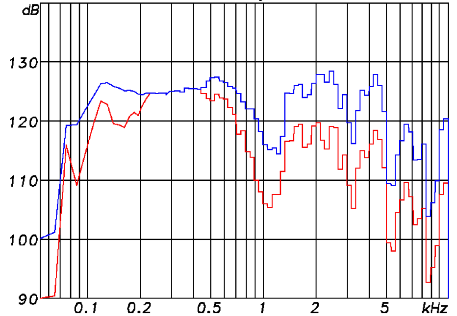
Max.SPL @ 3% 10% @ 1m THD M5 Seeburg acoustic line max. Power = 750W
