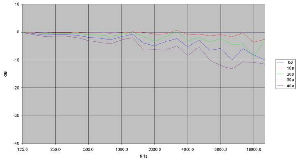
M5 Horizontal - Frequenzgang Off Axis+
