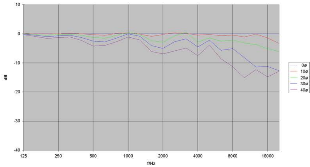
M5 Vertikal - Frequenzgang Off Axis+
