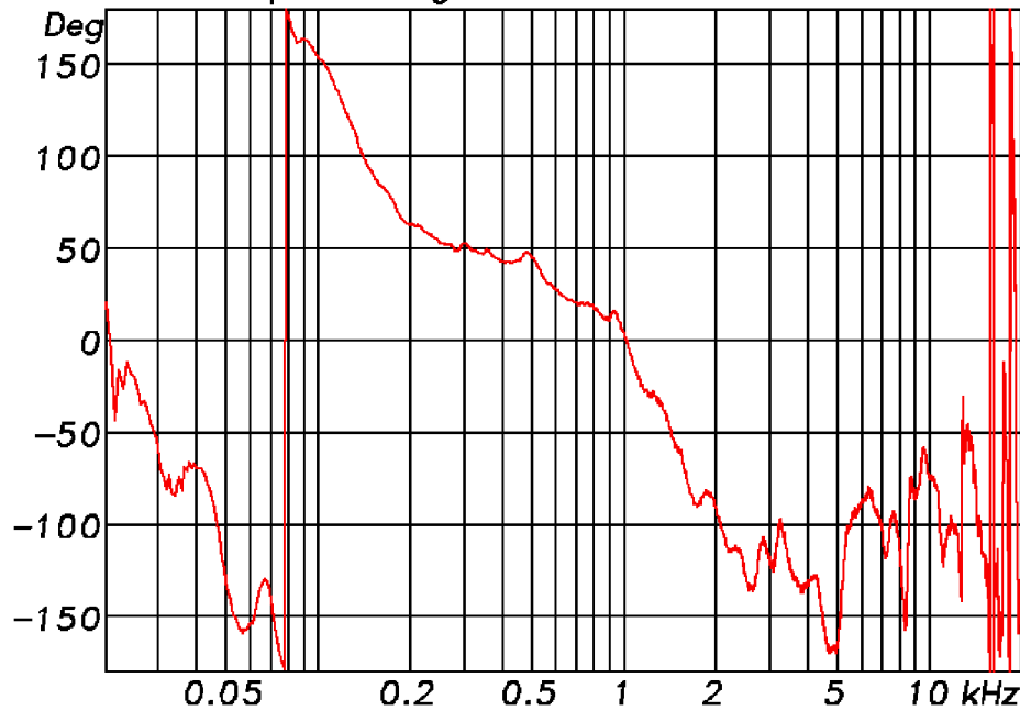
Phase Resp. Seeburg acoustic line M5
