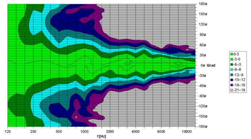
M5 Vertikal - Directivity Plot
