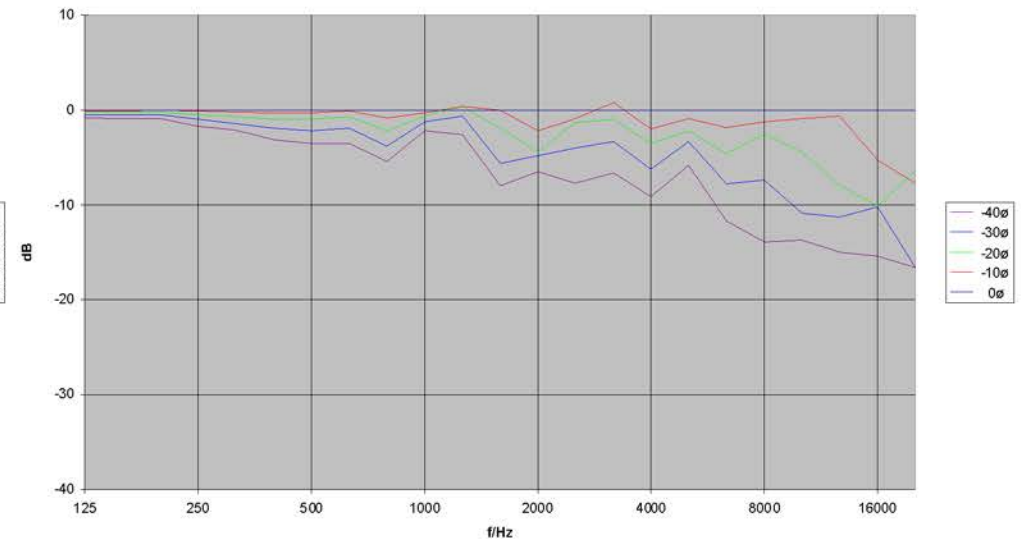
M5 Vertikal - Frequenzgang Off Axis-
