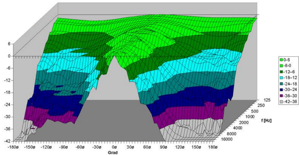
M5 Vertikal - 3D Directivity Plot
