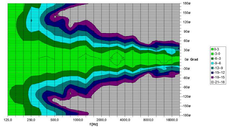
M5 Horizontal - Directivity Plot
