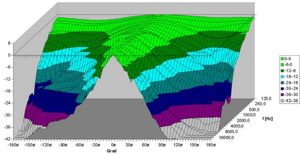
M5 Horizontal - 3D Directivity Plot
