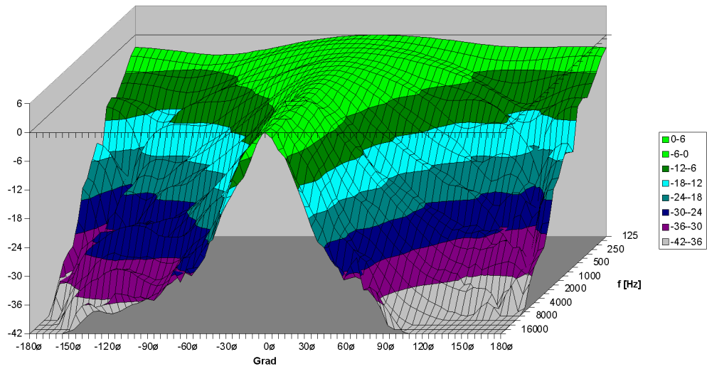
F8 60° x 50° Horizontal - 3D Directivity Plot
