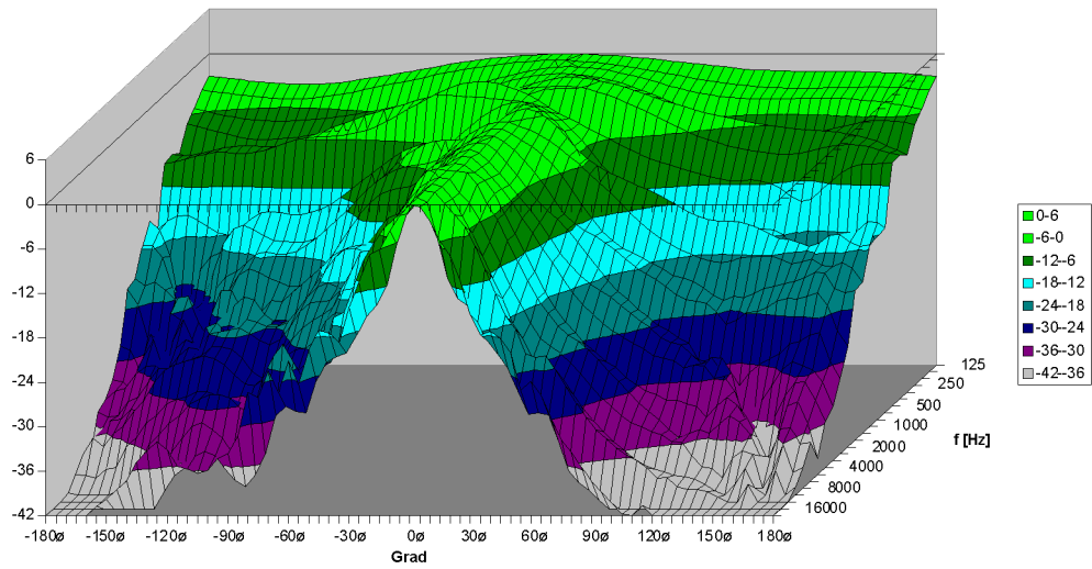
F8 60° x 50° Vertikal - 3D Directivity Plot
