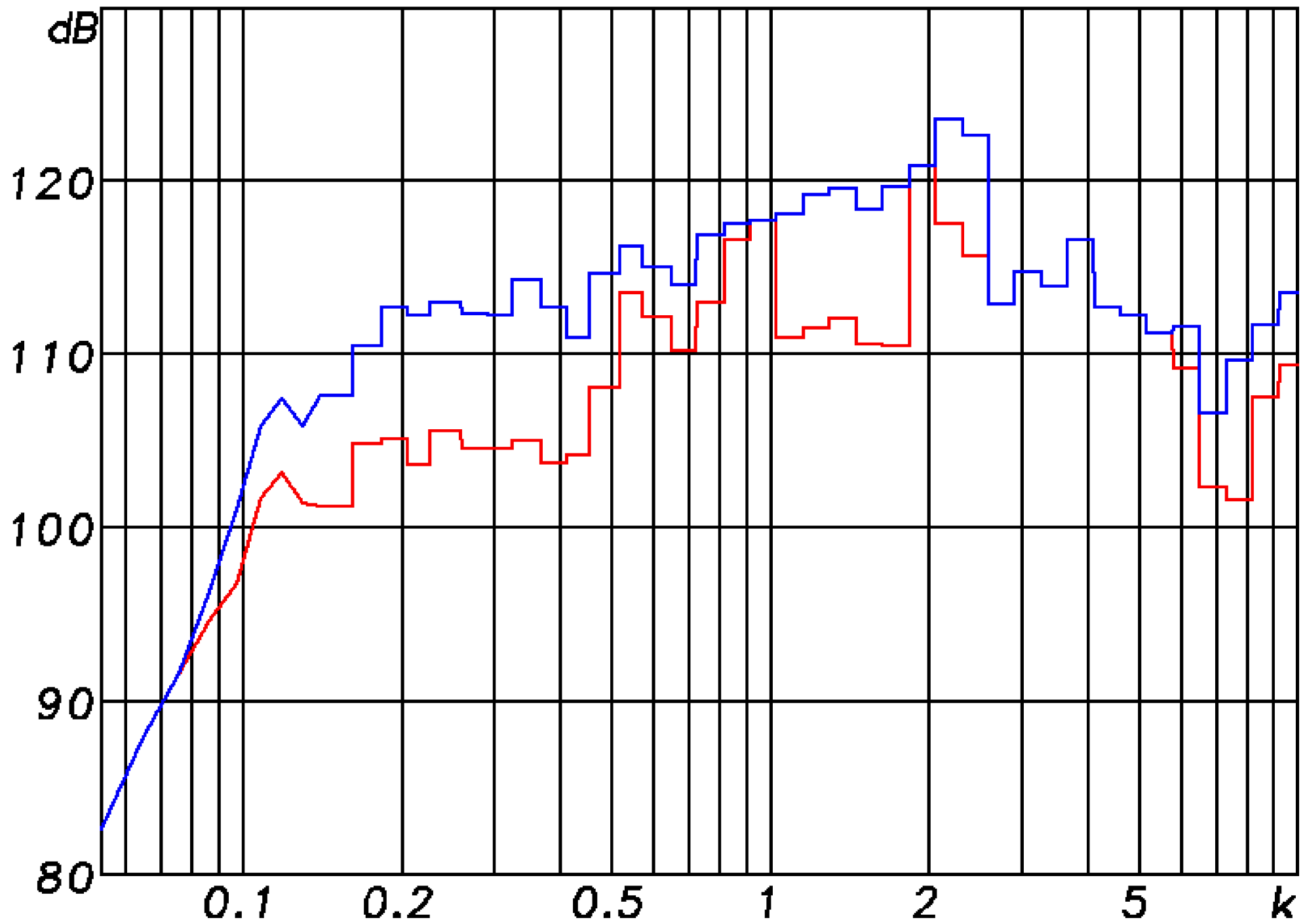
Max.SPL @ 3% und 10% THD A1 300W 80hm
