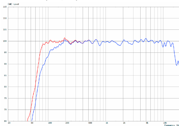
K 30 xov - Frequency Response with DSP Presets
