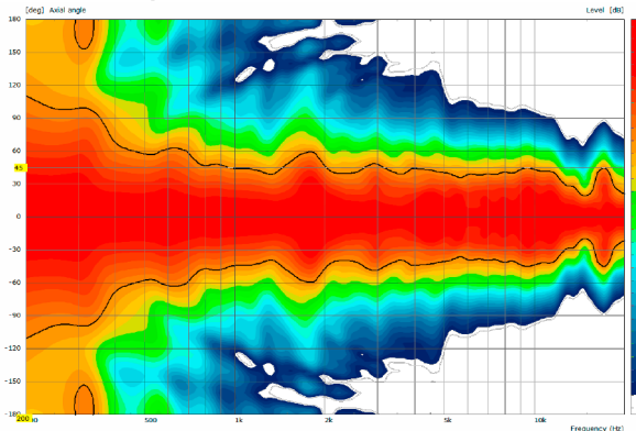
2D Directivity Plot - horizontal - 90° x 50°
