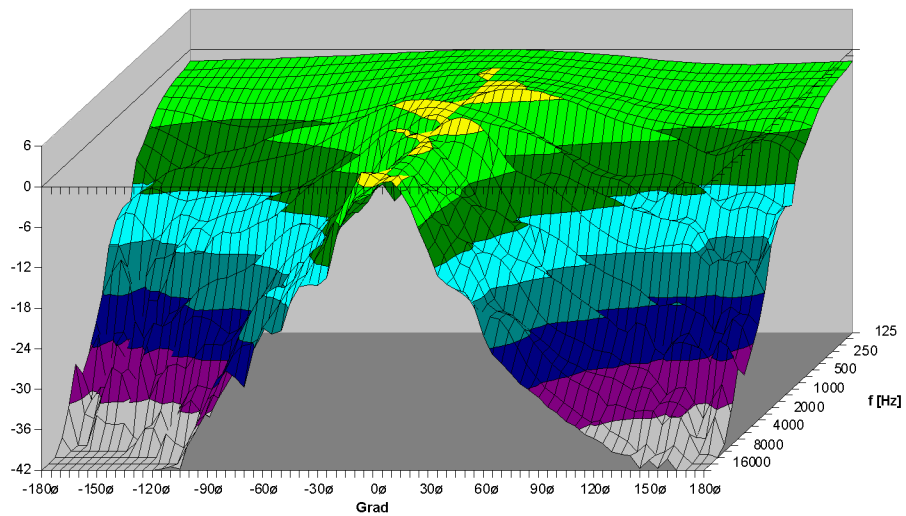
TSMini Vertikal - 3D Directivity Plot
