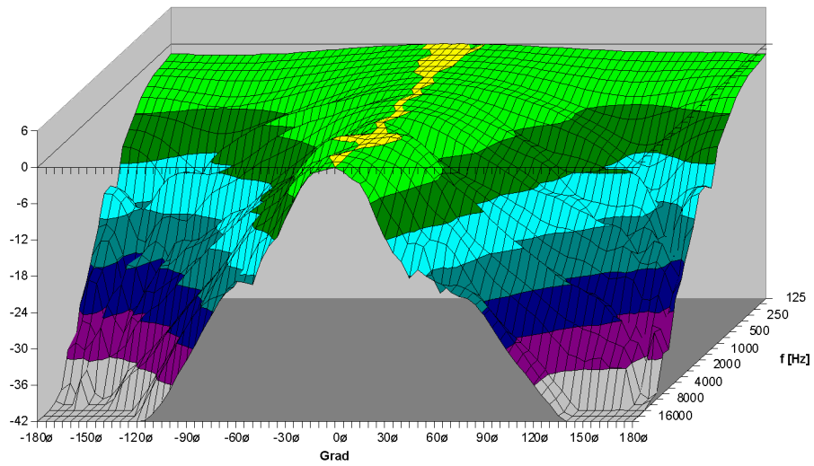
TSMini Horizontal - 3D Directivity Plot
