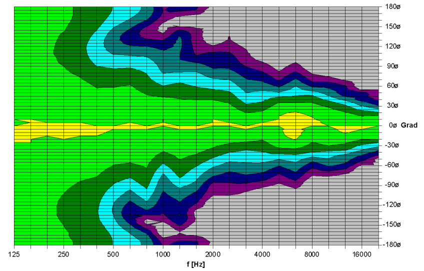
TSMini Horizontal - 2D Directivity Plot
