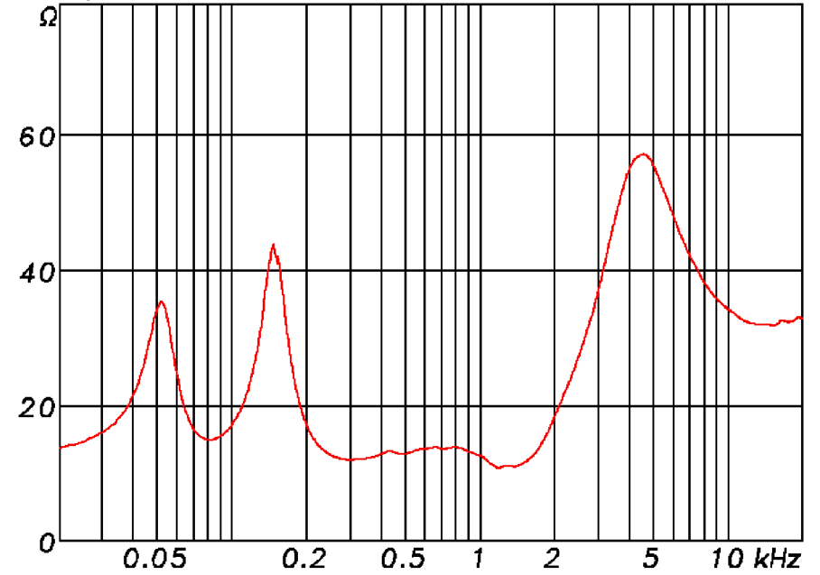
Impedance TS-Mini Norm.= 16 Ohm ; Min.= 10, 8 Ohm
