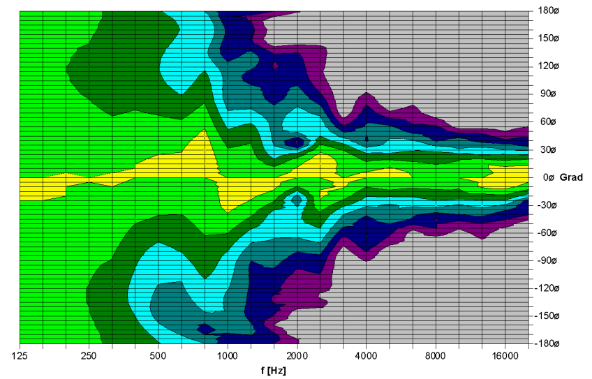
TSMini Vertikal - 2D Directivity Plot
