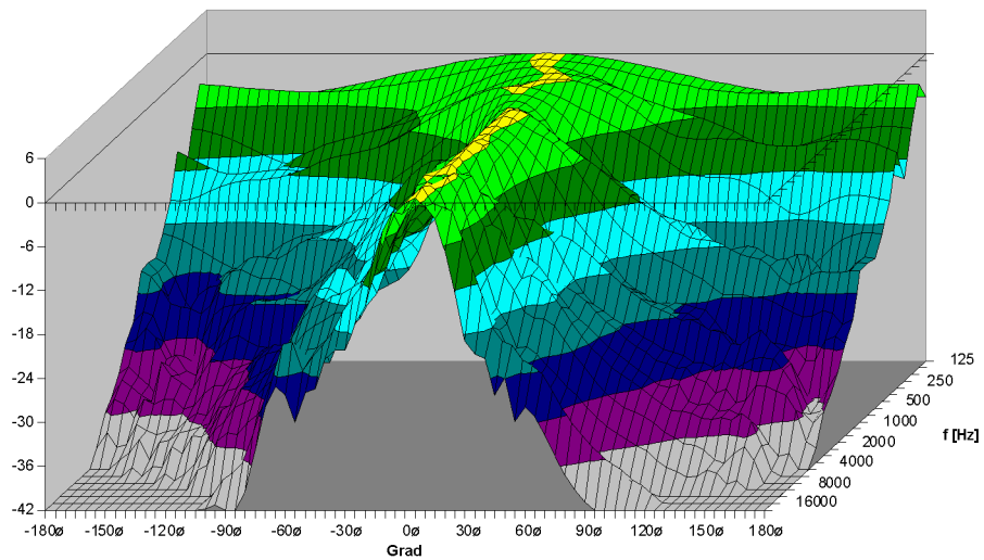
TSE 6040 Vertikal - 3D Directivity Plot
