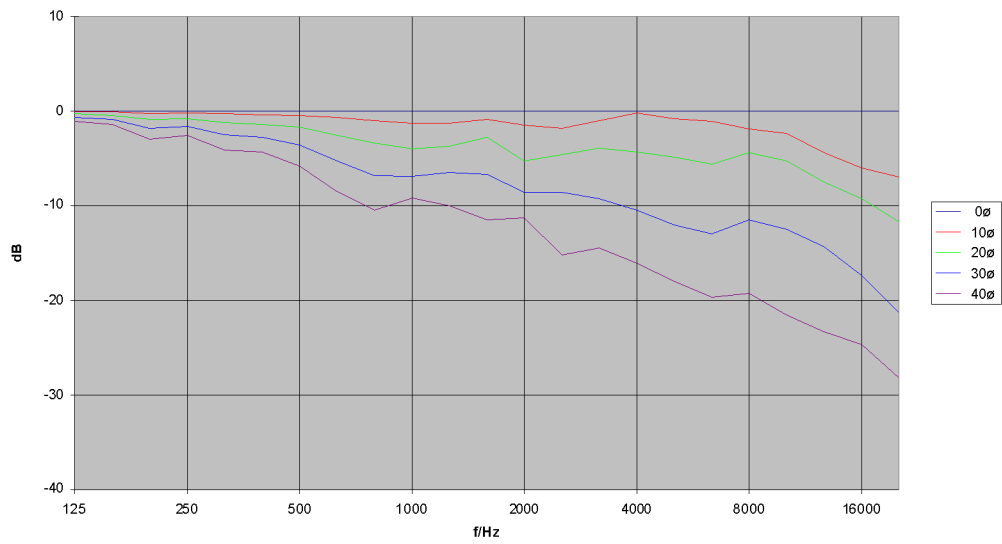
TSE 6040 Horizontal - Frequenzgang Off Axis (+)
