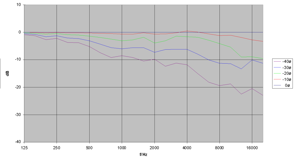
TSE 6040 Horizontal - Frequenzgang Off Axis (-)
