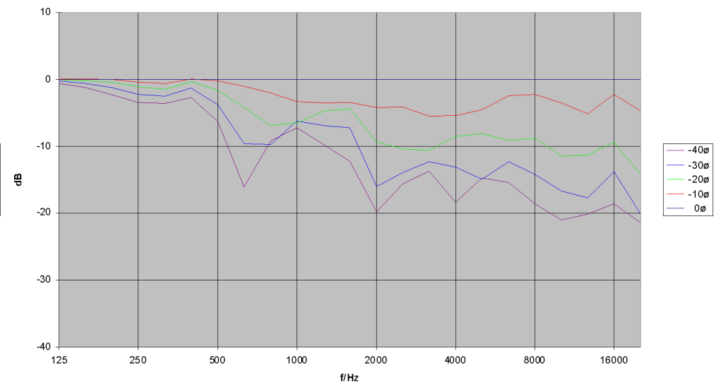
TSE 6040 Vertikal - Frequenzgang Off Axis (-)
