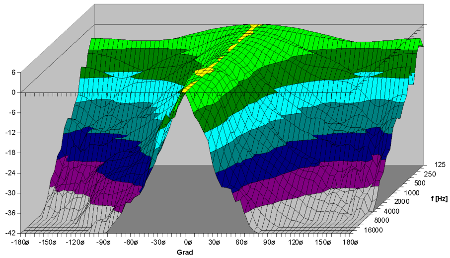
TSE 6040 Horizontal - 3D Directivity Plot
