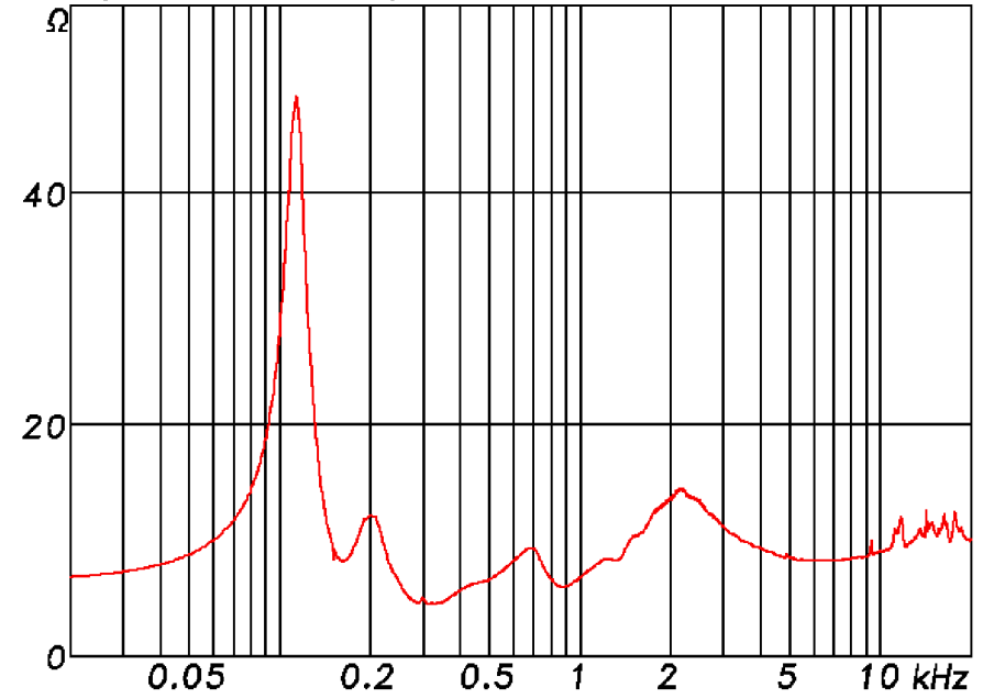
Impedance TSE6040/K2 Norm.= 8 Ohm Min.= 4, 5 Ohm
