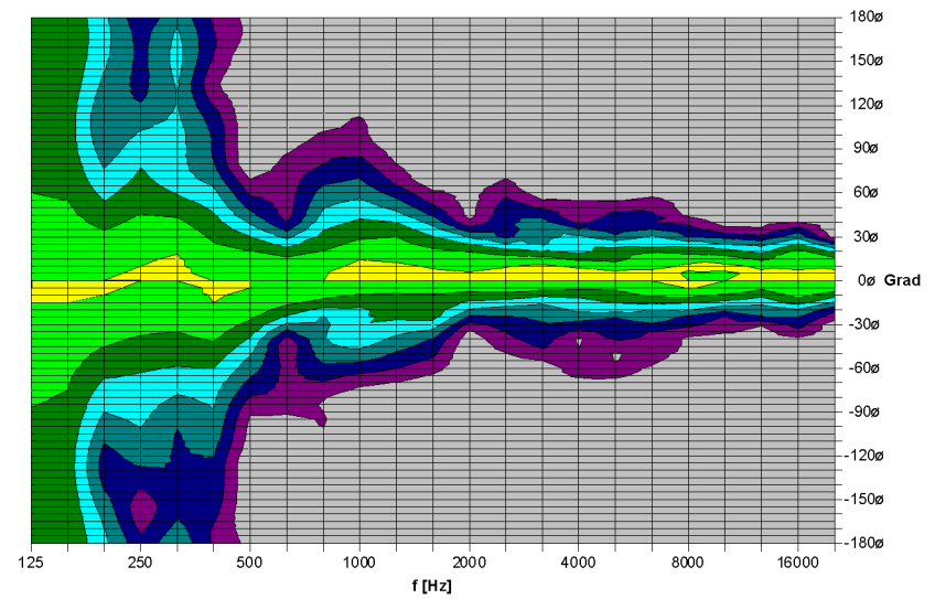
TSE 6040 Vertikal - 2D Directivity Plot
