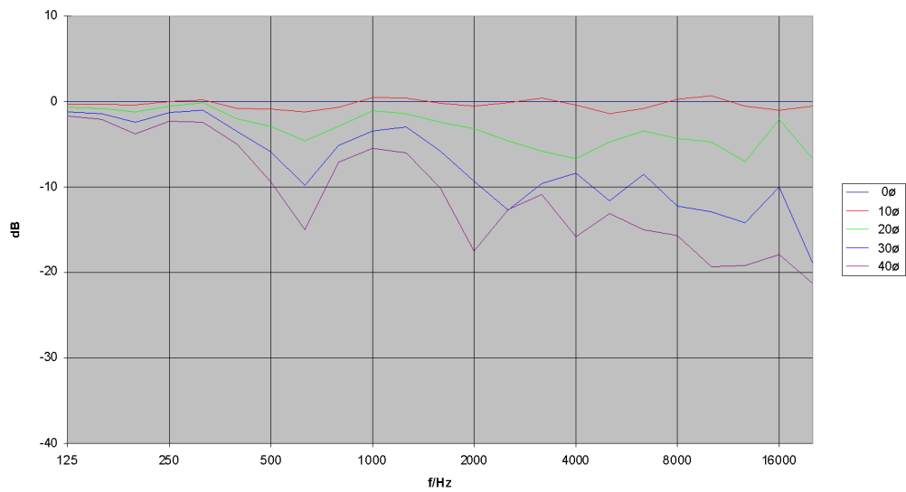
TSE 6040 Vertikal - Frequenzgang Off Axis (+)
