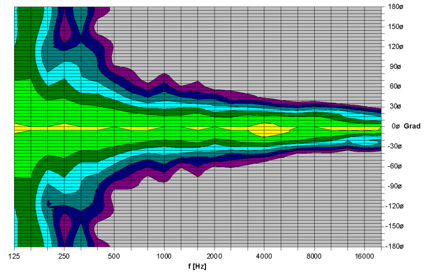
TSE 6040 Horizontal - 2D Directivity Plot
