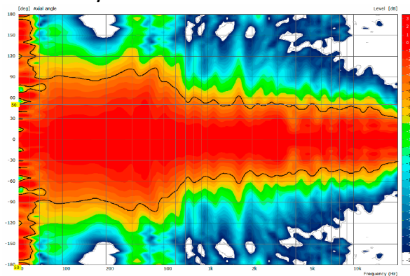
2D Directivity Plot - Cardioid Mode
