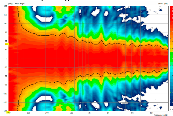
2D Directivity Plot - Hypercardioid Mode
