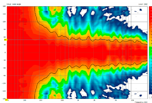
2D Directivity Plot - Endfired Mode
