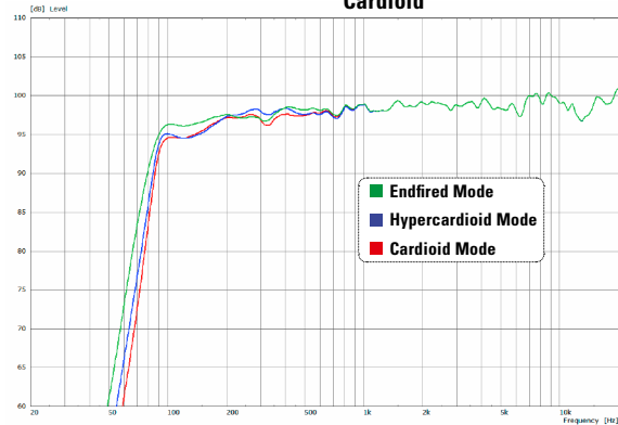
Frequency Response with DSP - Endfired, Hypercardioid + Cardioid
